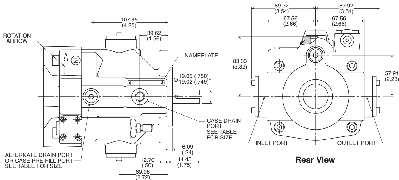
OPTION "B" SPLINE SHAFT SAE "A" 9T 16/32 DP 30° INVOLUTE SPLINE MAX TORQUE = 58.2 N-m (517 IN-LBS)
