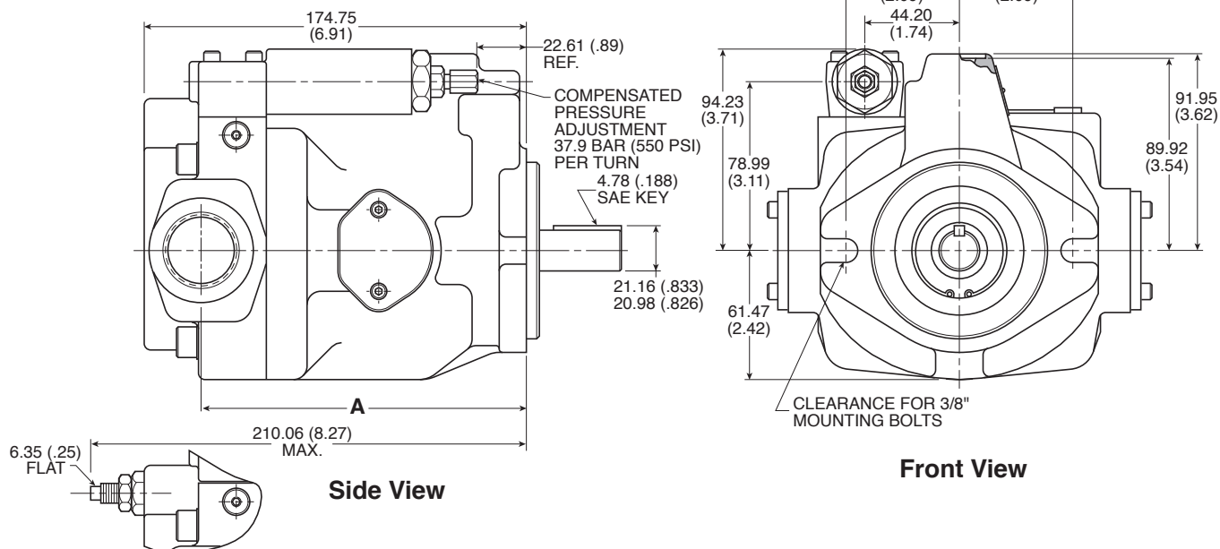
ADJ. MAX. VOLUME STOP (1.6 CC/REV/TURN) "OPTION 2"
